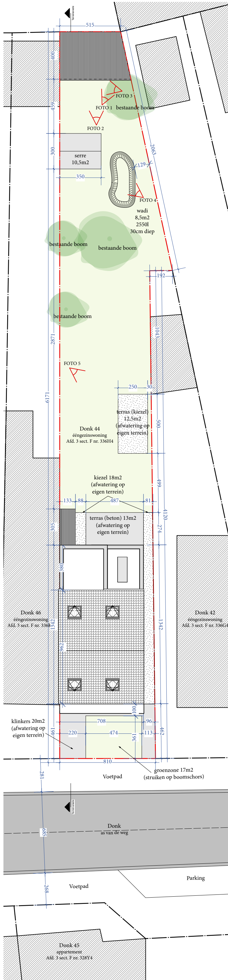
BA_2026-DONK_I_N_1_Inplantingsplan (piv2)
