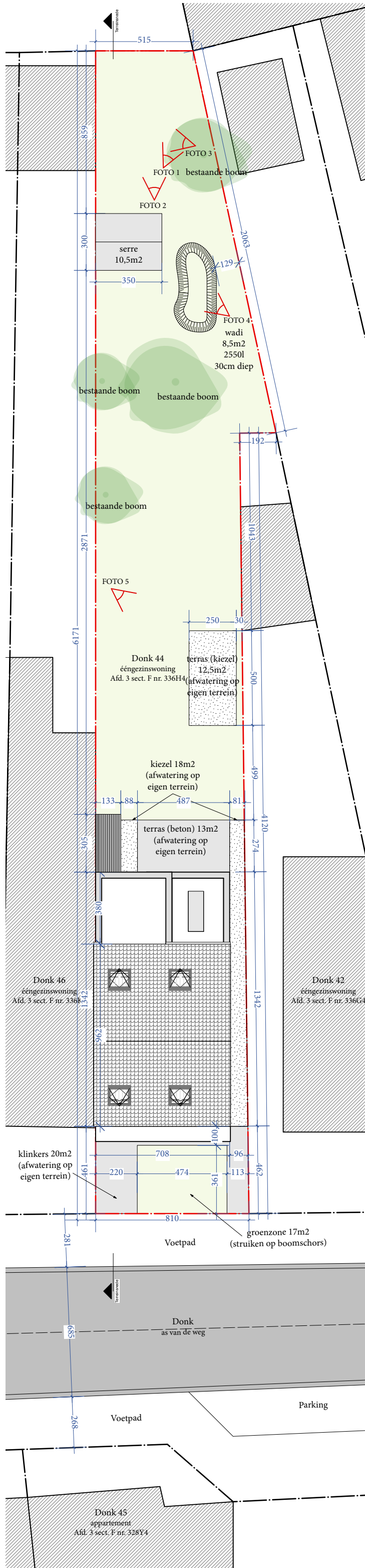
BA_2026-DONK_I_B_1_Inplantingsplan (piv 2)
